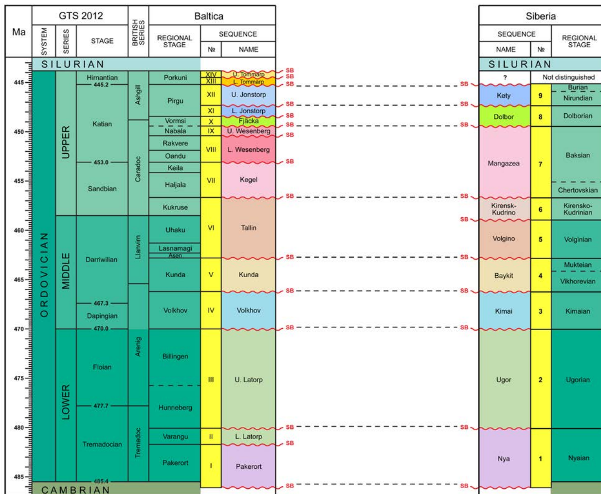
Fig. 5. Comparison the Ordovician sequence stratigraphic charts of Baltica and Siberia.
