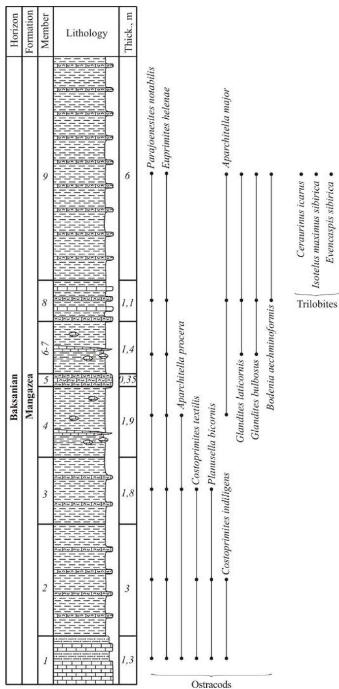
Fig. 35. Lithology and ranges of fossil taxa from the Outcrop-VI – the Podkamennaya Tunguska River, left bank, 2–3 km below Kuzmovka Village.
